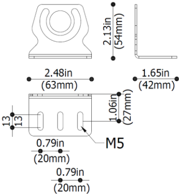
SYFX01 Side mounting brackets
